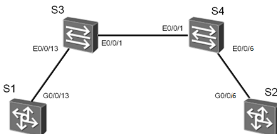
Figure 1.3 GVRP topology
