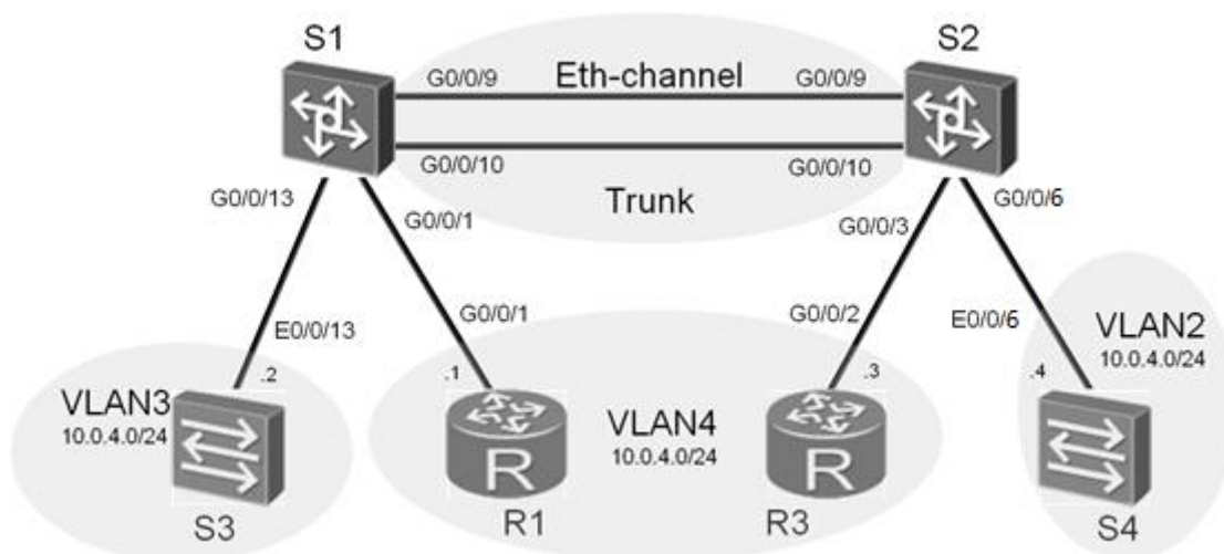
Figure 1.2 VLAN topology
