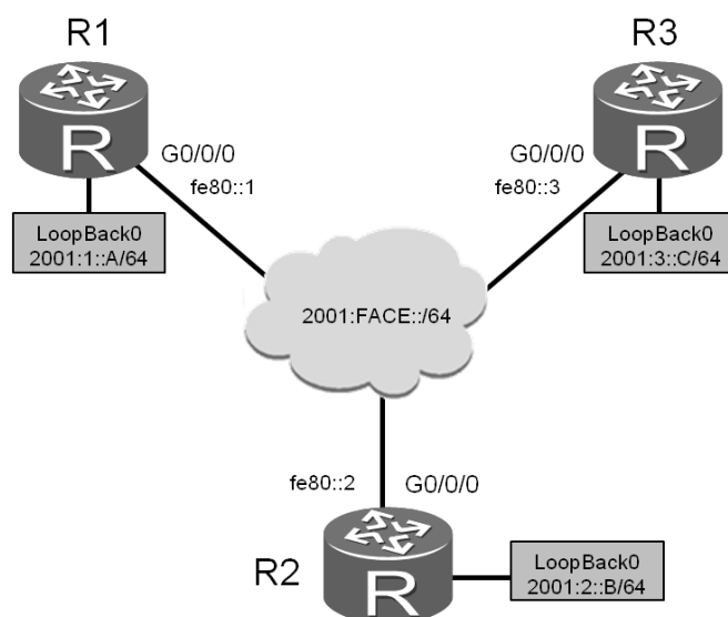
Figure 5-1 IPv6 topology
